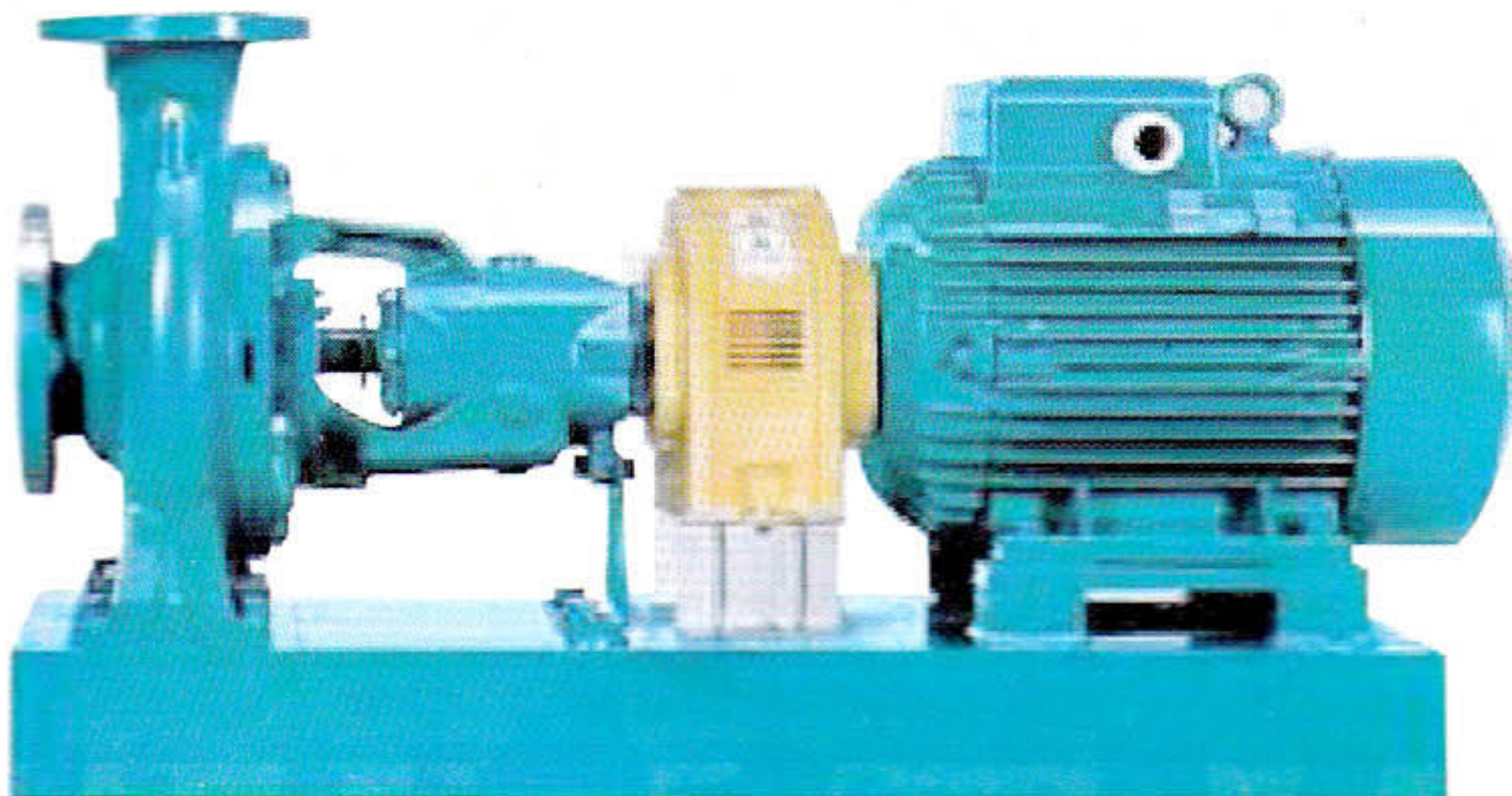
Electricity Driven Fire Pump/Centrifugal Fire Pump Origin Italy/Germany (Motor Driven)
