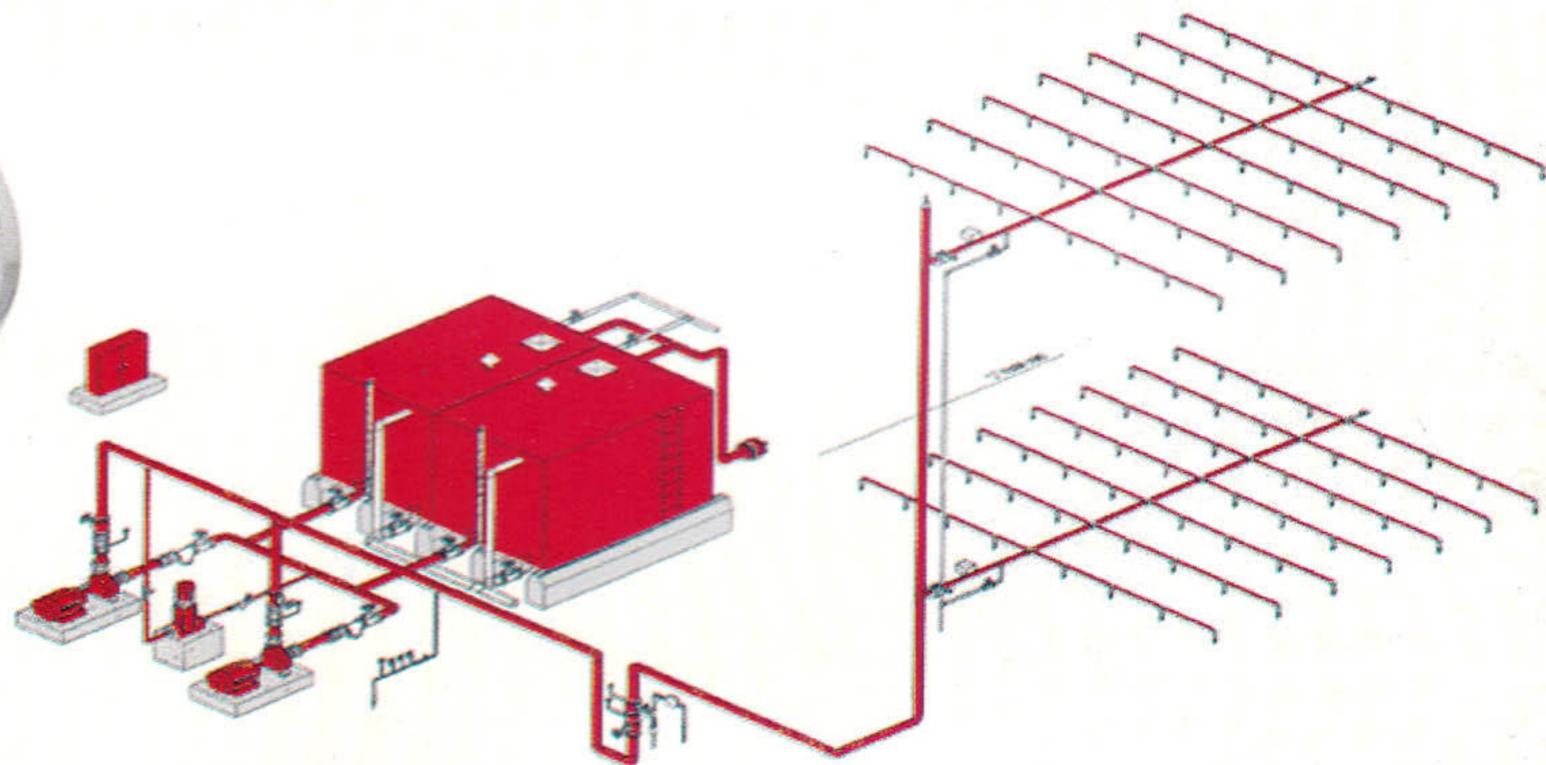
Sprinkler Model
